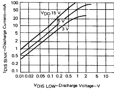
DISCHARGE CURRENT
